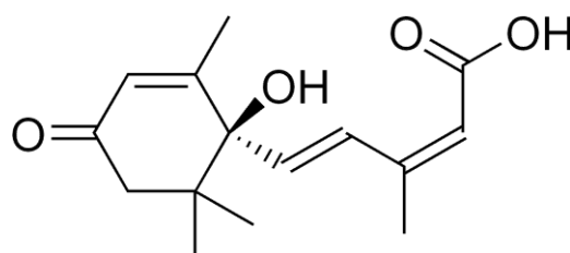
Fig- Structure of Abscisic acid
