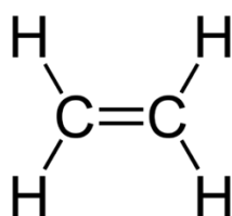
Fig- Structure of Ethylene
