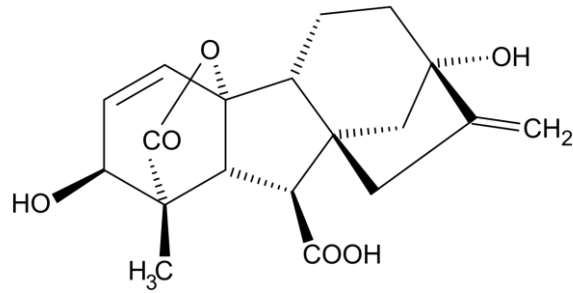
Fig- Structure of GA
